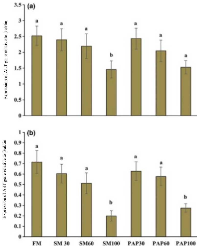
Figure 7: Expression of ALT (a) and AST (b) genes relative to \beta -aktin.
